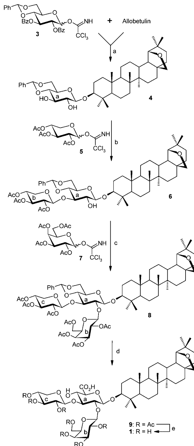
Scheme 1. Synthesis of target molecule 1 . Reagents and conditions: a) TMSOTf (0.05 equiv.), CH 2 Cl 2 ; NaOMe, MeOH/CH 2 Cl 2 (72%). b) TMSOTf (0.005 equiv.), IP, CH 2 Cl 2 , –75 \rightarrow –58 ^{\circ} C (73%). c) TMSOTf (0.03 equiv.), IP, CH 2 Cl 2 , room temp. (qu). d) EtSH, TsOH, CH 2 Cl 2 (89%); TEMPO, NaOCl, TBAC, KBr, CH 2 Cl 2 /H 2 O/NaHCO 3 (69%). e) NaOMe, MeOH/CH 2 Cl 2 . IR-120 (H + ) (qu).
