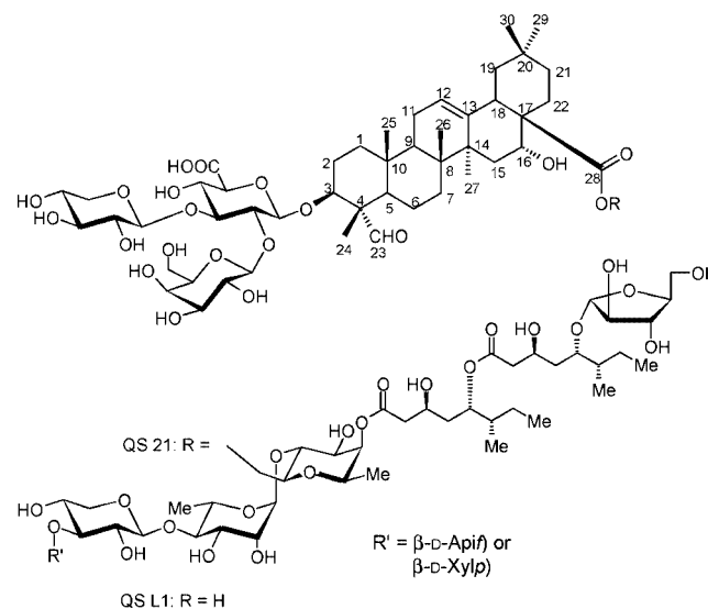
Figure 1. Structures of saponins QS 21 and QS L1.
