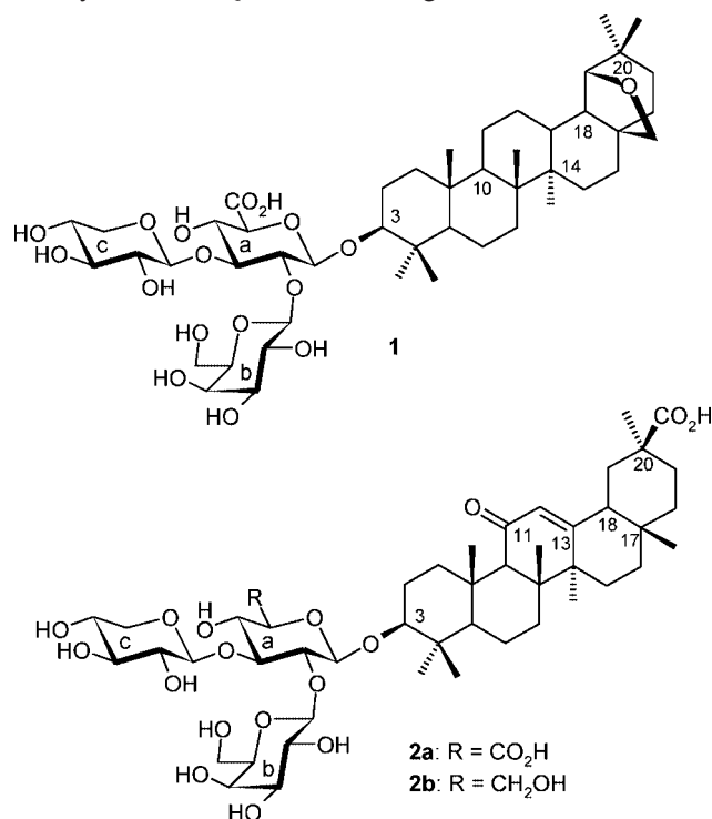
Figure 2. Structure of target molecules 1 , 2a and 2b .
