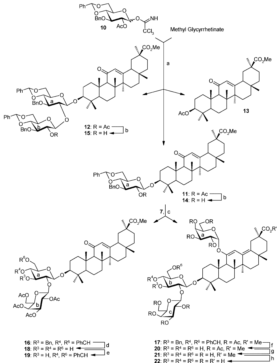
Scheme 2. Synthesis of intermediate 19 . Reagents and conditions: a) TMSOTf (0.06 equiv.), \text{CH}_2\text{Cl}_2 , room temp. ( 11 : 72%; 12 : 12%; 13 : 10%). b) NaOMe, MeOH, room temp. ( 14 : 95%; 15 : 95%). c) TMSOTf (0.05 equiv.), IP, \text{CH}_2\text{Cl}_2 , room temp. ( 16 : 85%; 17 : 5%). d) Pd/C, \text{H}_2 , MeOH/ \text{CH}_2\text{Cl}_2 (qu). e) PhCH(OMe) 2 , TsOH, MeCN, room temp. (85%). f) Pd/C, \text{H}_2 , MeOH/ \text{CH}_2\text{Cl}_2 (qu). g) KOH, EtOH/ \text{H}_2\text{O} , room temp., 16 h (qu). h) KOH, EtOH/ \text{H}_2\text{O} , refl, 3 h (70%).
