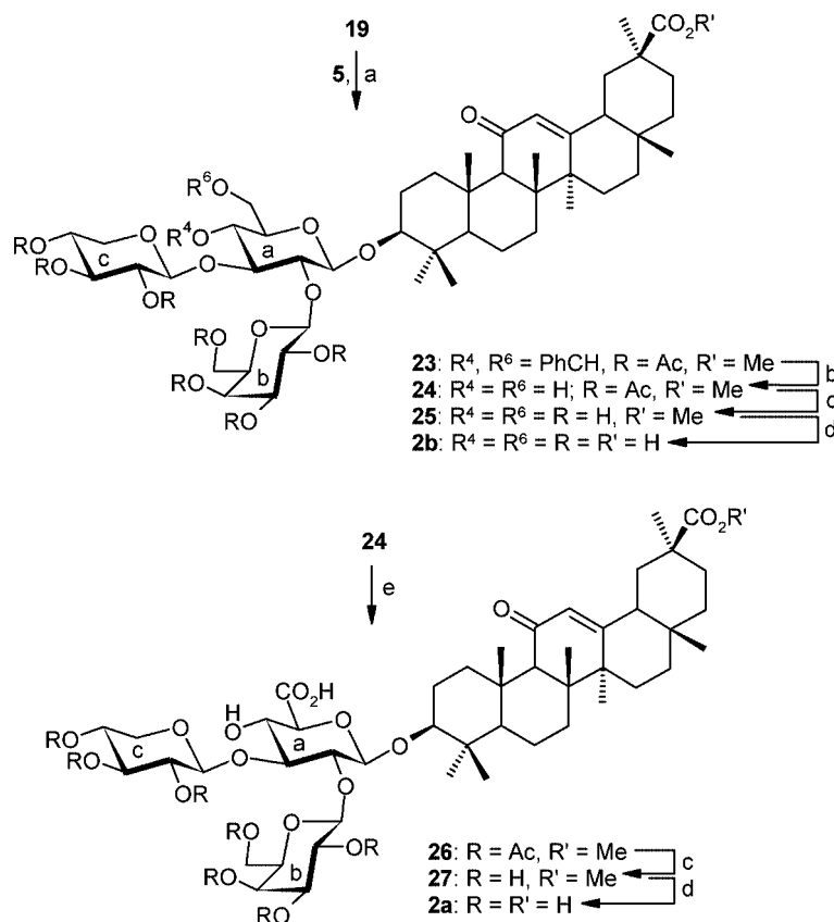
Scheme 3. Synthesis of target molecules 2a and 2b . Reagents and conditions: a) TMSOTf (0.05 equiv.), CH 2 Cl 2 , room temp. (86%). b) EtSH, TsOH, CH 2 Cl 2 , room temp. (83%). c) NaOMe, MeOH (qu). d) LiOH, MeOH, 54 °C ( 2b : 75%; 2a : 55%). e) TEMPO, NaOCl, TBAB, NaBr, CH 2 Cl 2 /H 2 O/NaHCO 3 (75%).
